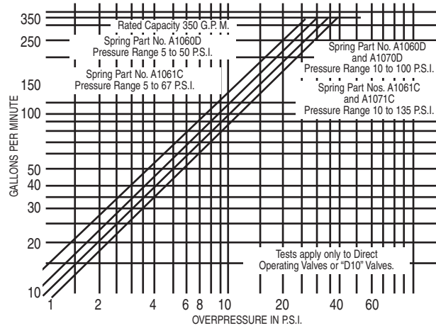
3" VALVE TESTS
