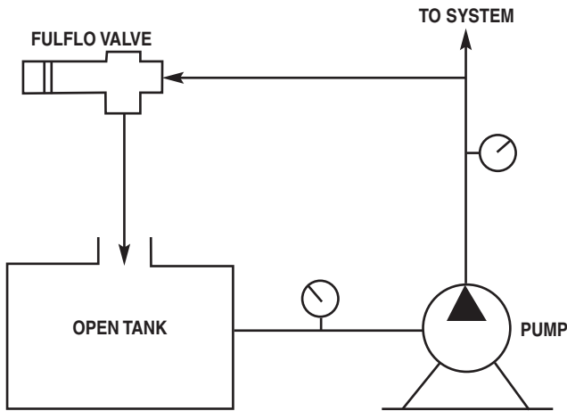
OPEN TANK
