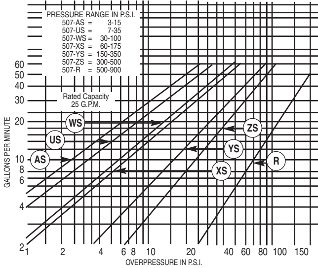
1" VALVE TESTS
