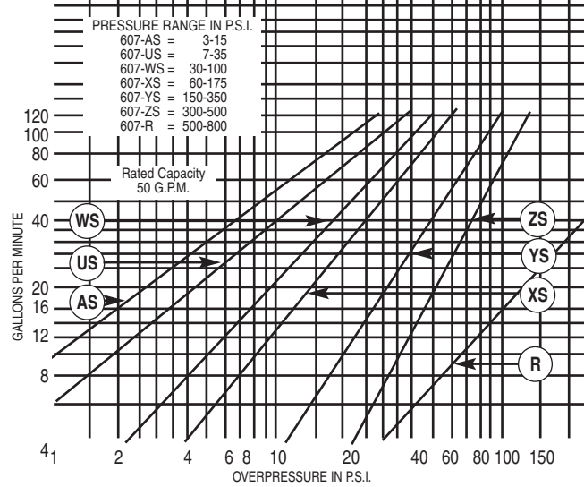
1 1/2" VALVE TESTS
