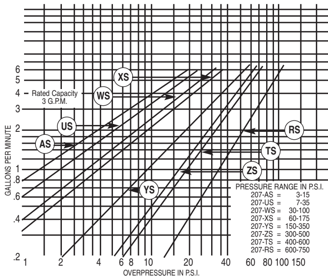
1/4" VALVE TESTS
