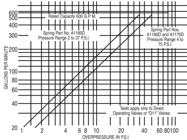
4" VALVE TESTS
